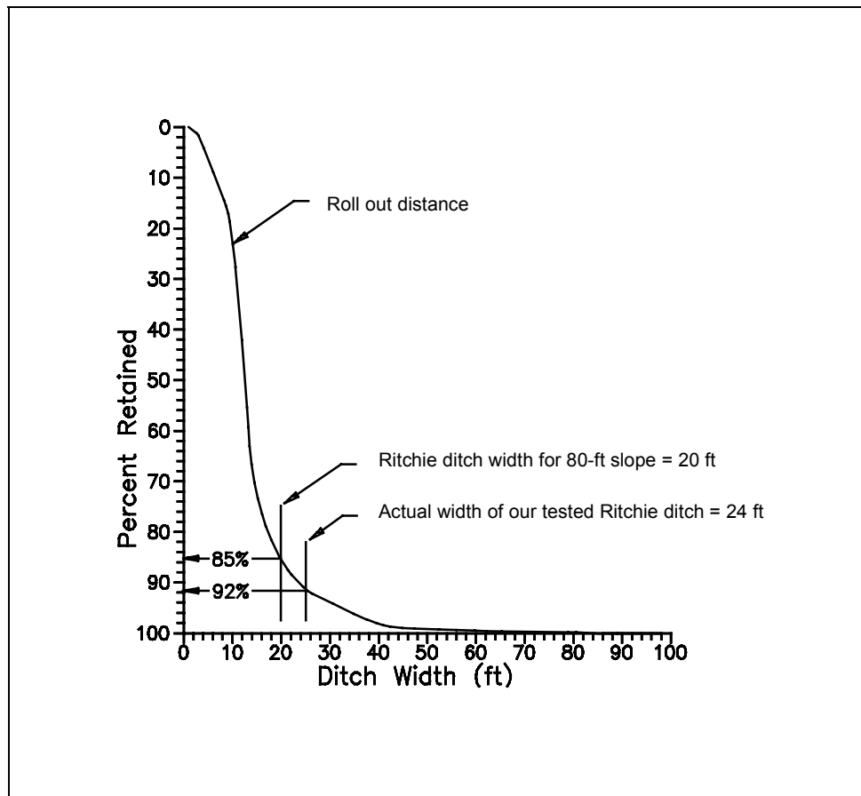
Figure 2.6: Cumulative percentage rockfall retained for tested Ritchie catchment area
